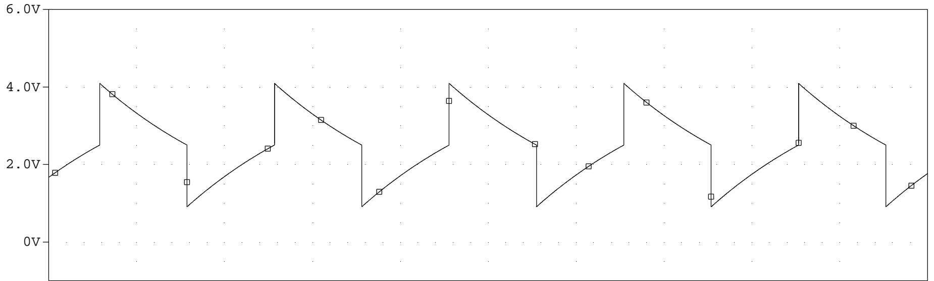
(A) Oscillator4.dat with Divider
