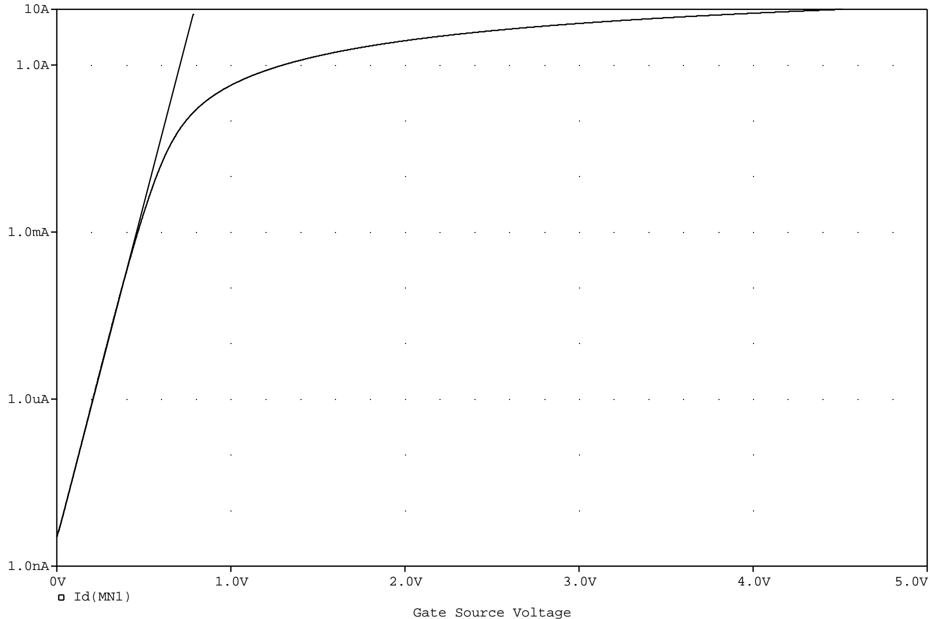
Test Log Behavior of ID Versus Gate Voltage, with VDS=+5V
