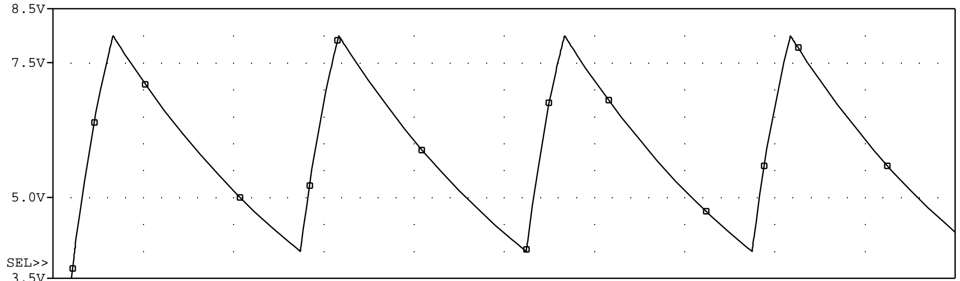
LM555, 4mS Up, 20mS Down (Approx.)
