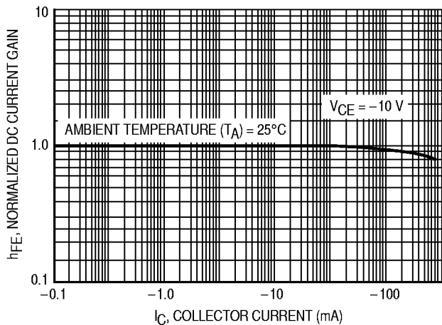
Figure 1. Current Gain Characteristics versus Collector-Emitter Voltage
